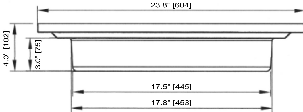
Part # STAR-18P
