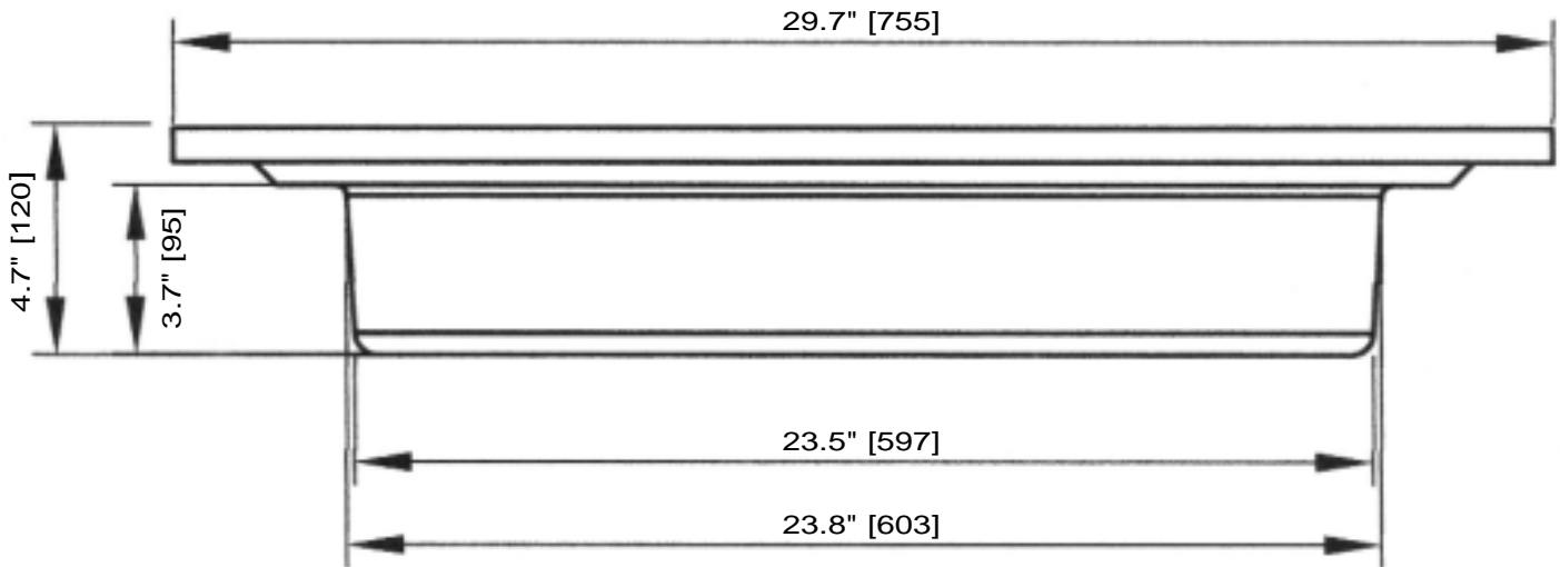
Part # STAR-24P
